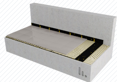
Limmade golv concrete slab + adhesive + Stravifloor Mat-F3 e + adhesive + final floor
