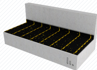
Ej limmade golv concrete slab + vapor barrier + Stravifloor Mat-F3e
