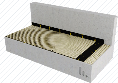
Limmade golv concrete slab + adhesive + Stravifloor Mat-F3 e + adhesive
