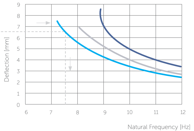
Deflection as Function of Frequency
