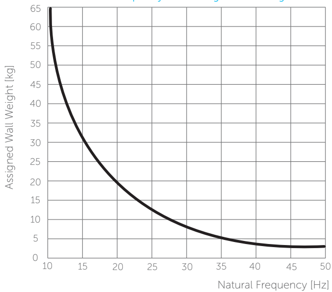
Natural Frequency under Assigned Wall Weight
