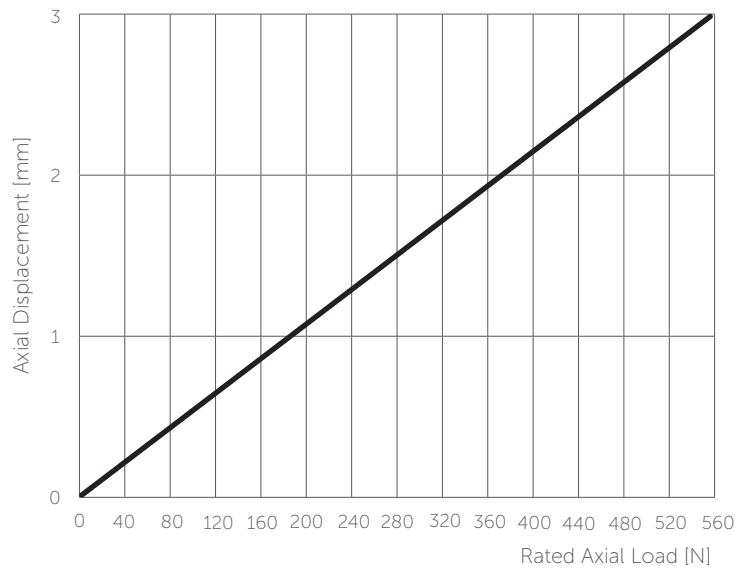
Rated Axial Load and Deflection
