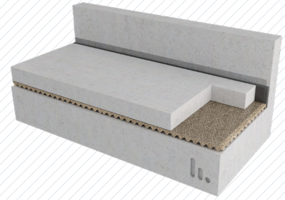
1 layer of Stravifloor Mat-W x
