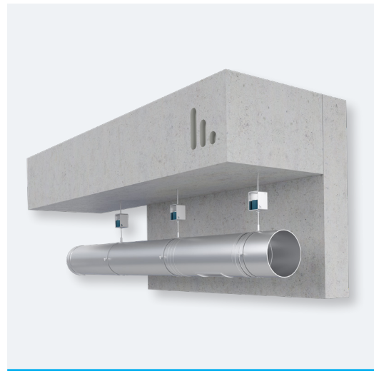
Figure 9 - Visual representation demonstrating the suspension of pipes using Stravilink ISH-P hangers.
