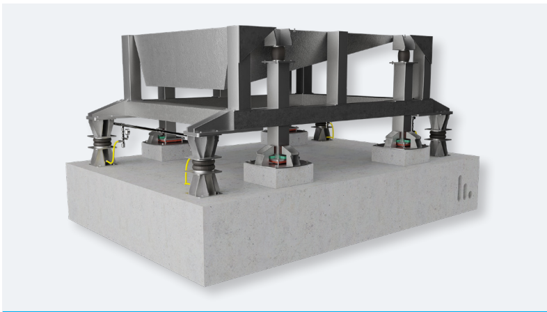
Figure 4 - Graphic representation of machine isolation at 'Adega Cooperativa de Alijó' (PT)
