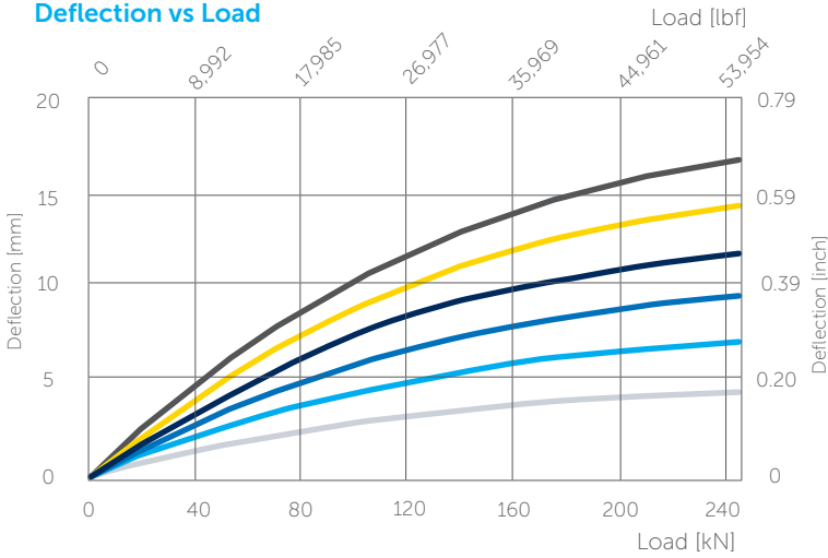
Deflection vs Load
