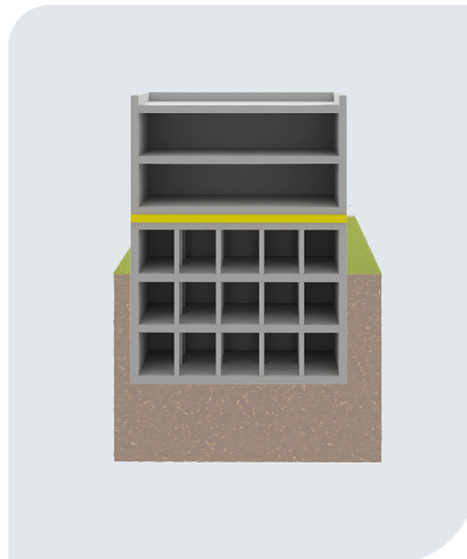
Figure 1.2 - Decoupling at floor level
