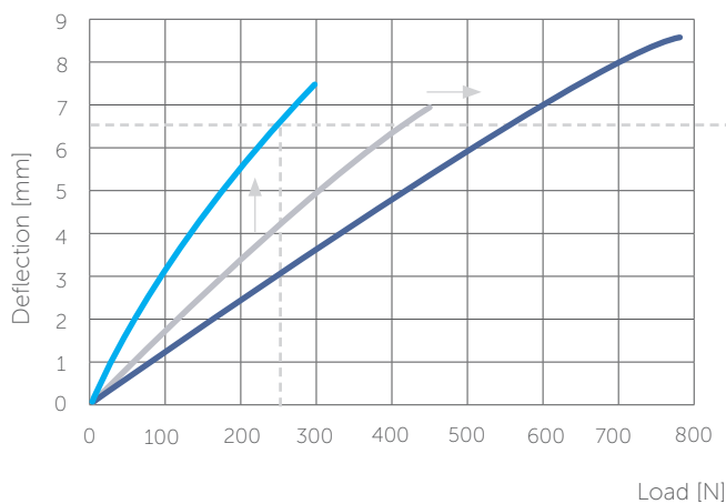
Deflection as Function of Load
