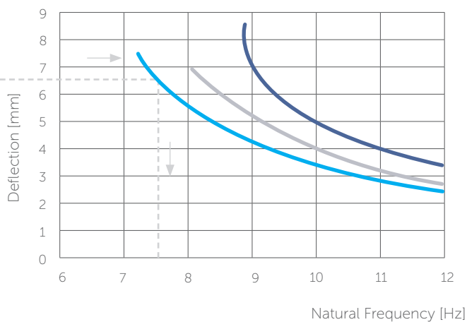
Deflection as Function of Frequency
