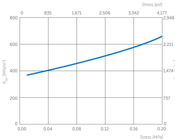
Dynamic Stiffness vs Stress
