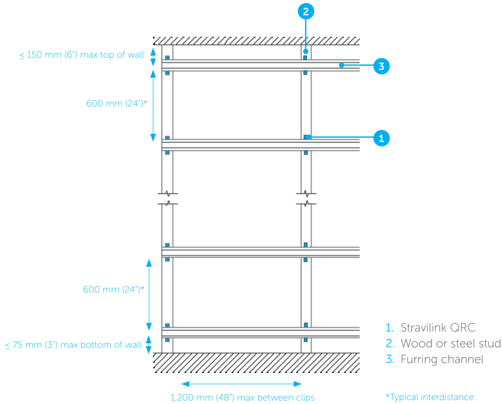
Typical wall elevation with Stravilink QRC and furring channel:
