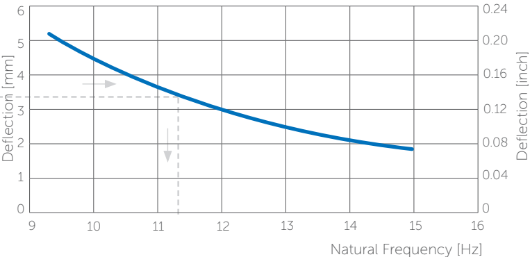
Relationship between Deflection and Natural Frequency
