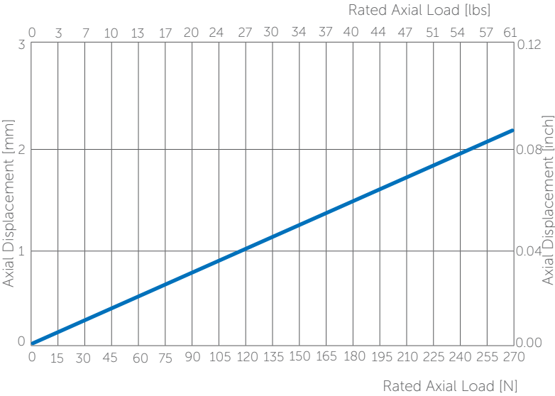
Rated Axial Load and Deflection
