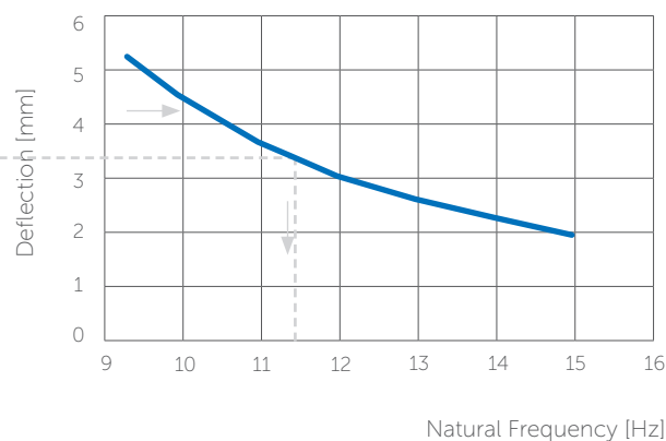
Relationship between Deflection and Natural Frequency
