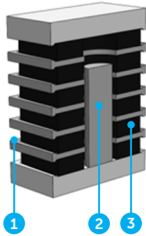
Stravibase VHS with integrated failsafe (VHS-FS)
