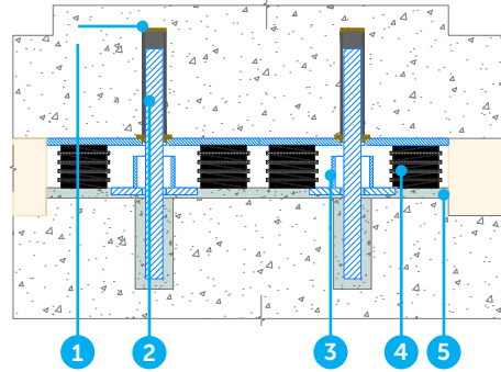
Stravibase VHS with shear dowels & failsafes
